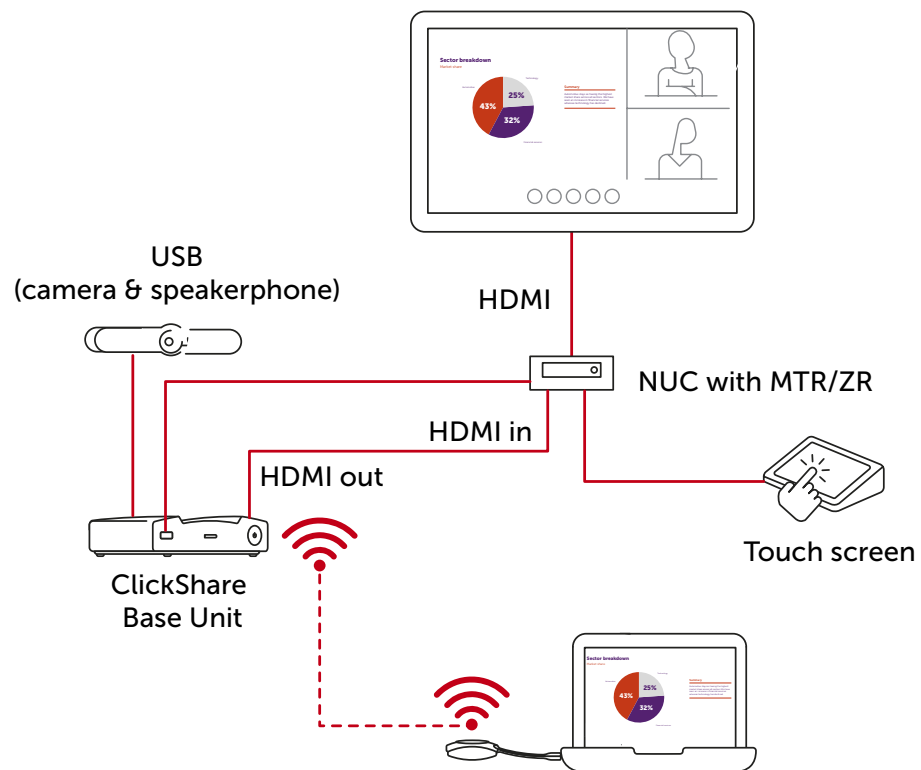
Automatic switching with ClickShare in a modular meeting room setup
