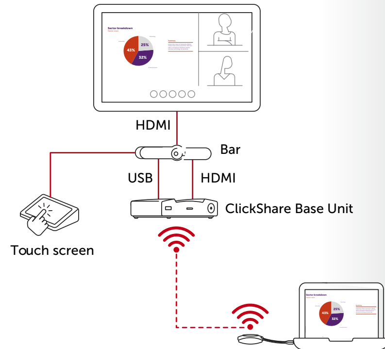
Automatic switching with ClickShare in an Android meeting room setup
